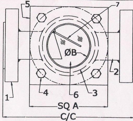
FLAPPER TYPE
