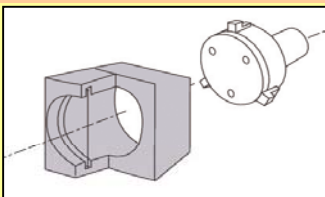
Internal Grooves
