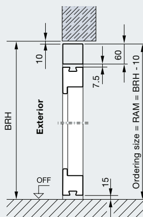
Vertical view Example: fitting in the opening
