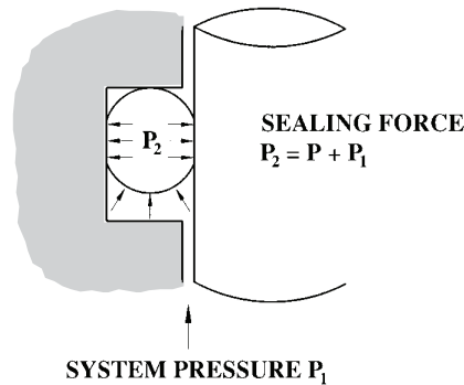
Figure 3: 'O' ring in typical housing
