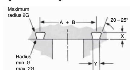
Figure 12: Dovetail groove
