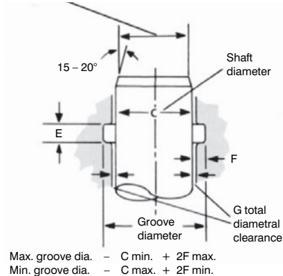
Figure 5: Plug groove, terminology as figures 4 and 13
