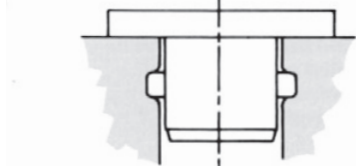
Figure 5: Plug groove, terminology as figures 4 and 13
