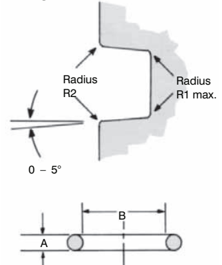
Figure 13: Groove radii and taper for figures 4-10
