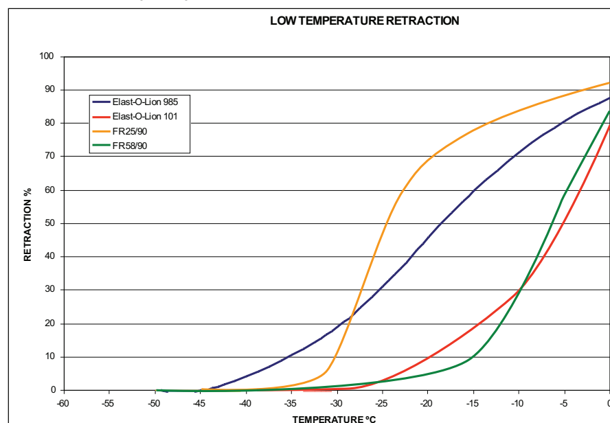
Figure 2: Comparative temperature retraction curves for four of James Walker's RGD-resistant elastomers at atmospheric pressure
