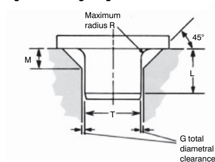
Figure 11: Triangular groove
