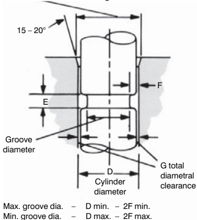
Figure 6: Groove in piston
