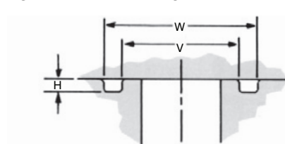
Figure 10: Groove in flange, Chart 72
