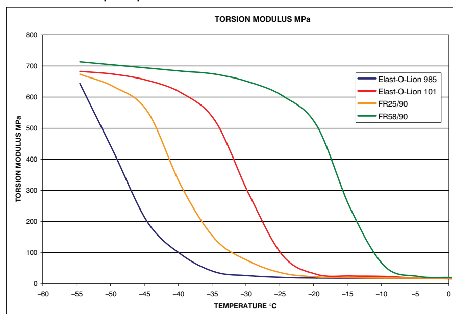
Figure 1: Comparative torsion modulus curves for four of James Walker's RGD-resistant elastomers at atmospheric pressure
