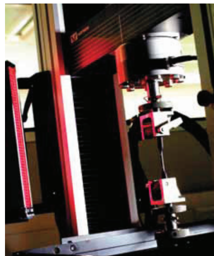
State-of-the-art visual extensometer for tensile testing elastomers
