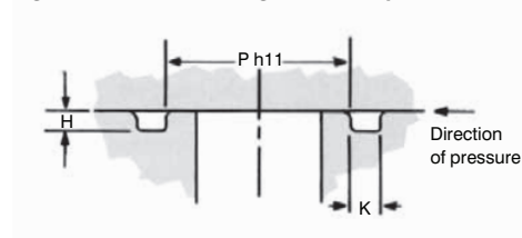
Figure 9: Groove in flange, internal pressure
