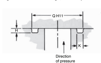
Figure 9: Groove in flange, internal pressure
