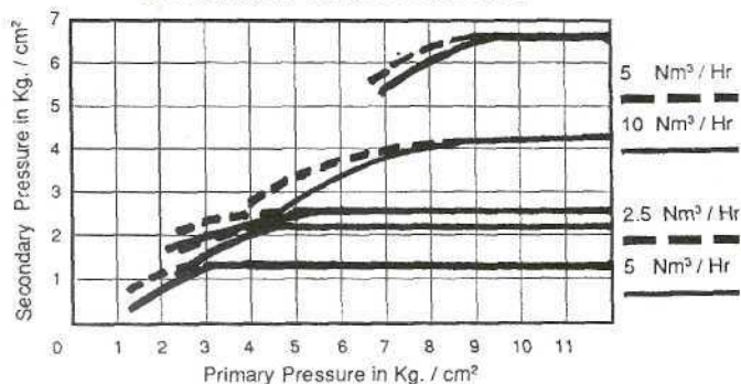
REGULATOR FLOW CHARACTERISTIC
