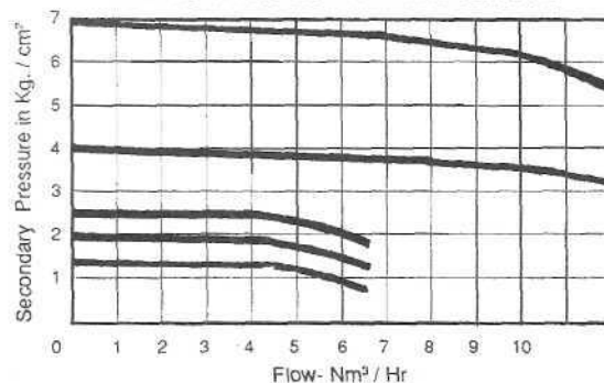
REGULATOR FLOW CHARACTERISTIC
