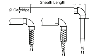
Straight End With Copper Elbow and Braid/Conduit
