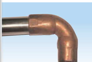
Straight End With Copper Elbow and Braid/Conduit
