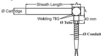
Square End with Conduit
