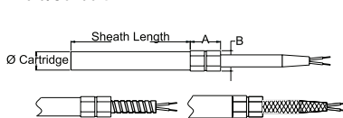
Straight End With Copper Coupler and Braid/Conduit
