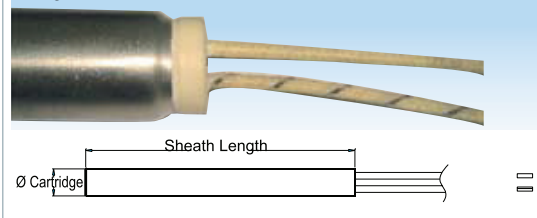
Swaged in Leads
